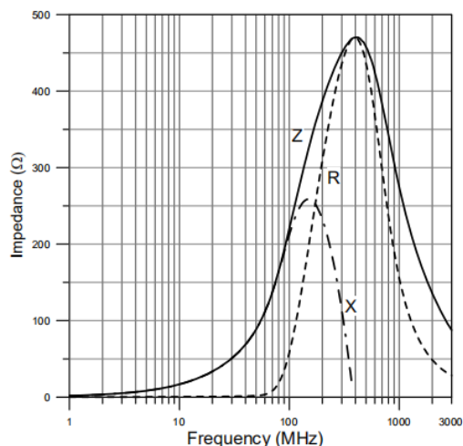
ECMS321608K102 4P
