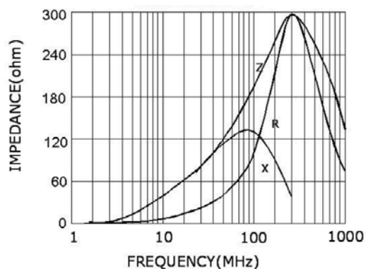
ECMS321608A121 4P
