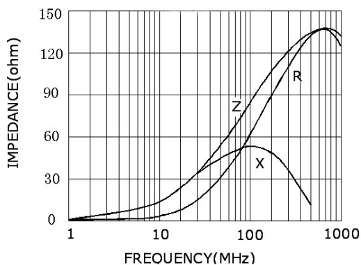
ECMS321608A600 4P
