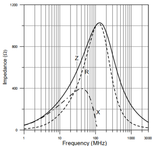
ECMS321608B601 4P
