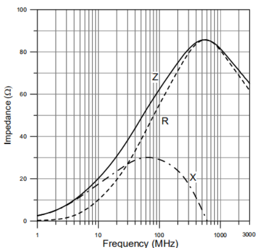
ECMS321608A301 4P
