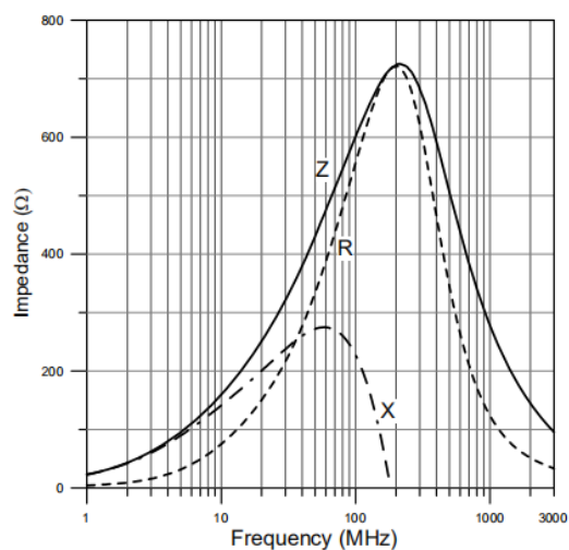
ECMS321608B221 4P
