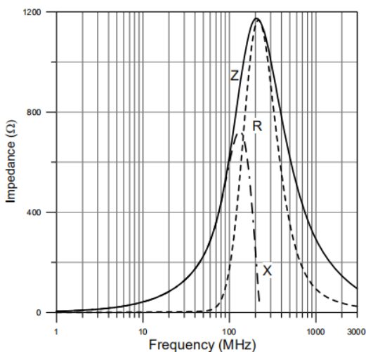
ECMS321608H121 4P
